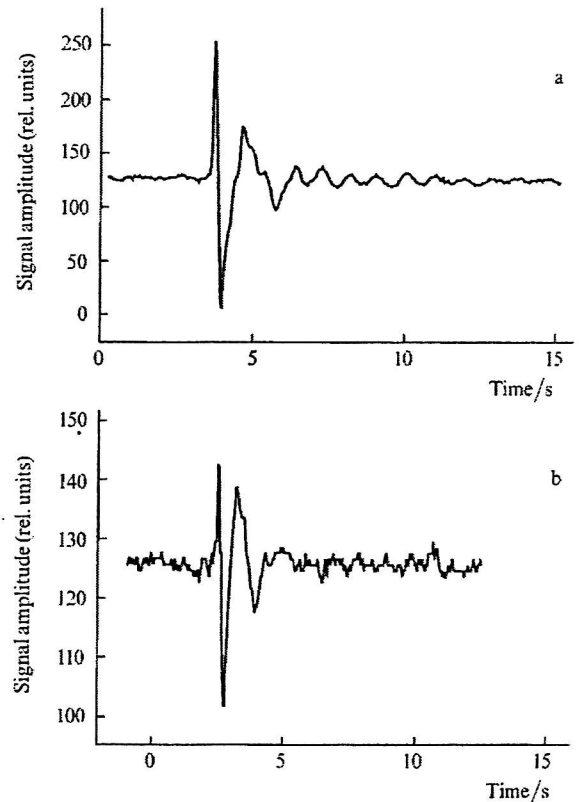
Figure 3. Optoacoustic response of the cartilage at the beginning (a) and at the end (b) of irradiation by a holmium laser ( E = 23 mJ, \tau = 0.3 ms, f = 20 Hz, t_{\text{exp}} = 7 s).
