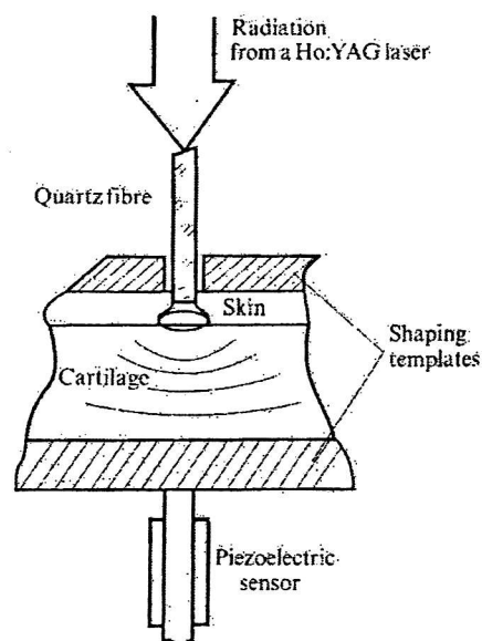
Figure 1. Scheme of laser correction of the shape of the porcine conch.
