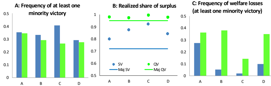
Figure 2: Bootstrap results . In panel A, the frequency is significantly higher for SV under rules B, C, and D ( p < 0.01 ; one-sided Z test). In panel B, none of the differences in means are statistically different from one another. Note the difference in surplus under majority in the SV and QV samples. In panel C, all frequencies are significantly positive, but smaller than 0.05 for SV-C (0.019) and SV-B (0.047).
