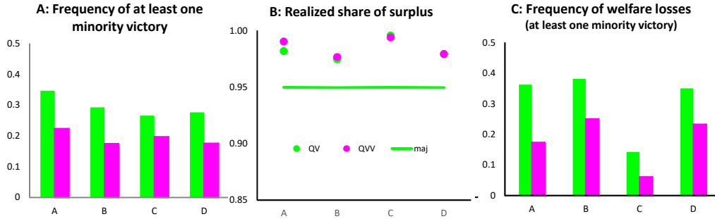
Figure 12: Bootstrapping the original QV sample: QV and QVV. The fractions of samples with at least one minority victory (Panel A) or with welfare losses, conditional on at least one minority victory (Panel C) are consistently lower under QVV ( p < 0.001 in all cases). In Panel B, the average shares of surplus are not statistically different from majority (based on bootstrapped CI's). All tests of proportions are one-sided Z tests.
