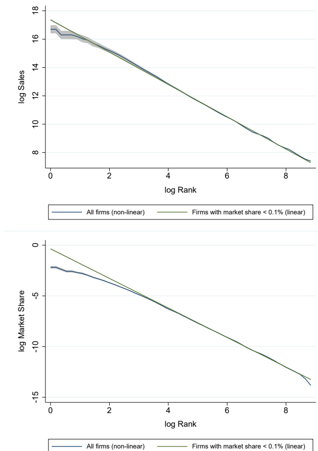
Figure 2: Size vs Rank Relationship (logs)
