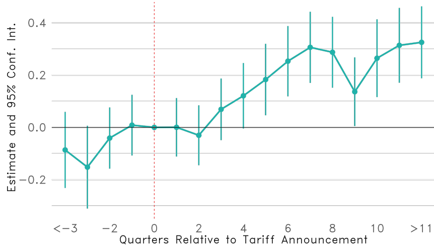
Figure 6: Province-level Rerouting
