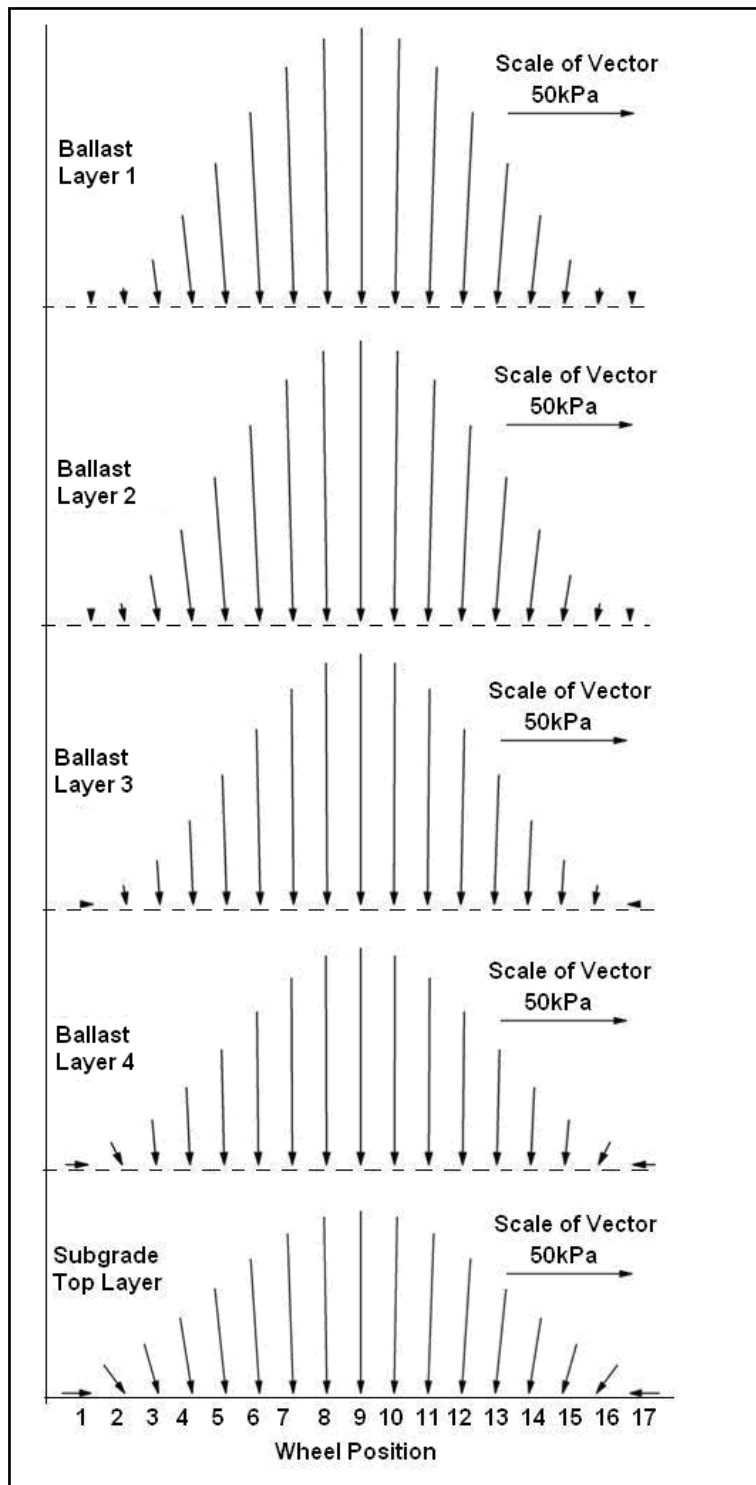
Figure 6.27 Major principal stress development in different analysis points under a moving wheel load
