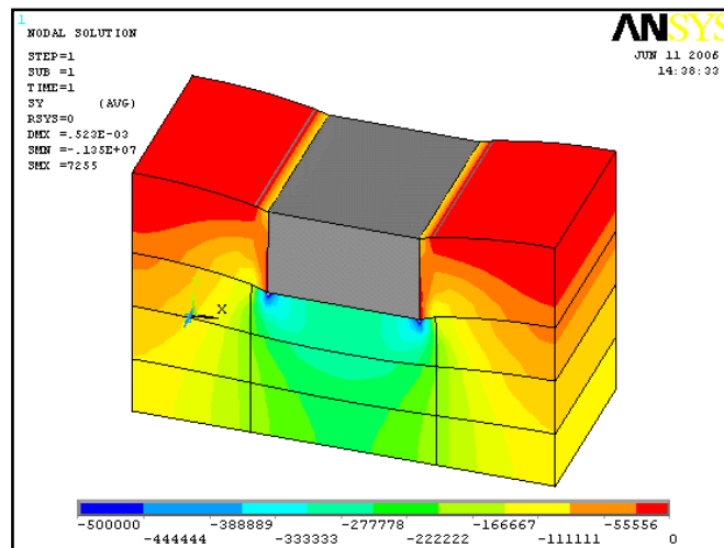
Figure 6.4 Vertical stress distribution in the box test simulation (Unit: Pa)
