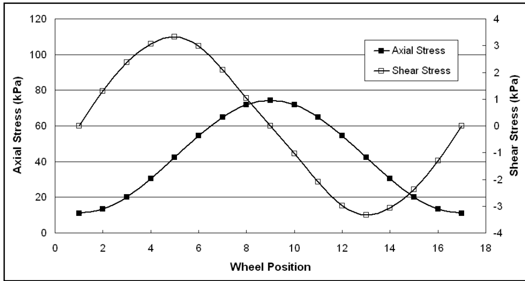
Figure 6.28 (e) Axial and shear stresses at the analysis point in subgrade layer under a moving load
