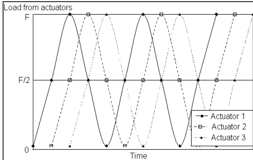
Figure 5.2 Loading pattern used in this project
