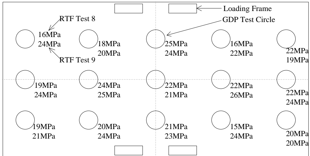
Figure 5.8 Subgrade stiffness measured by GDP
